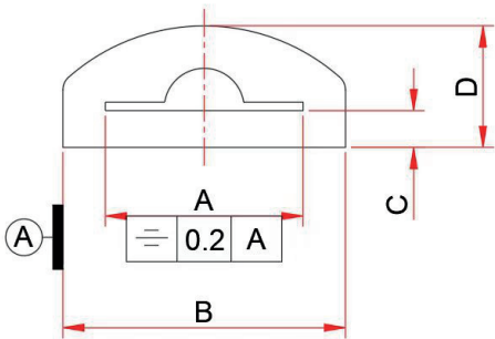
密封胶尺寸参考 Size reference after the strip light is glued
