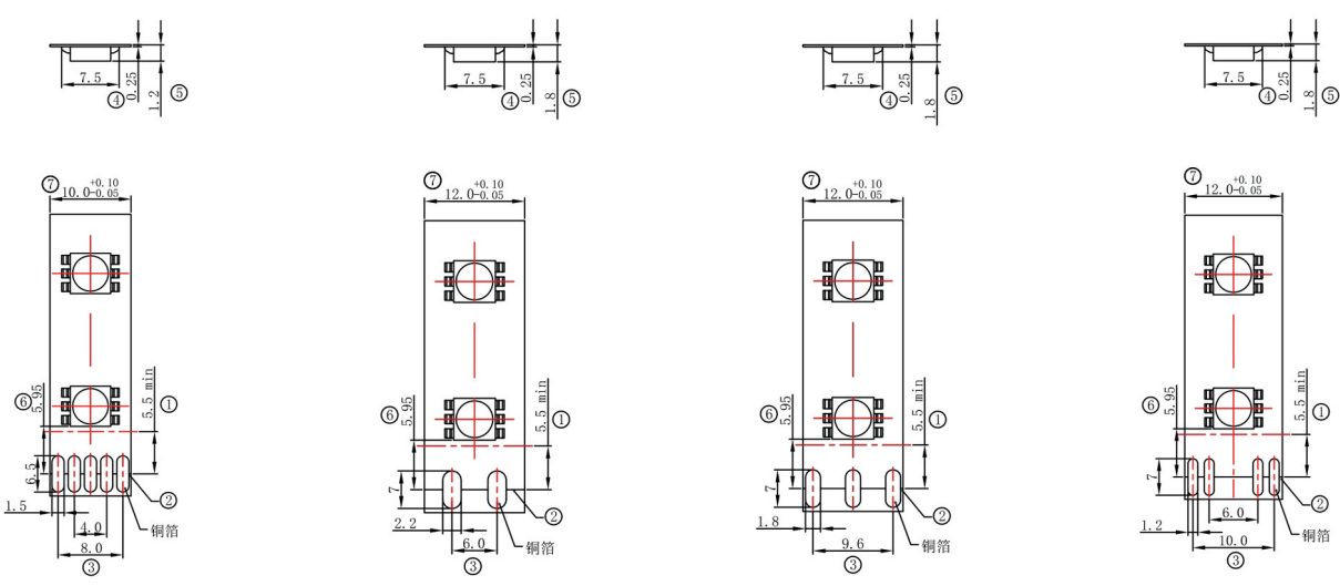
HR-IP-SMD-5PIN-10MM HR-IP-SMD-2PIN-12MM HR-IP-SMD-3PIN-12MM HR-IP-SMD-4PIN-12MM
