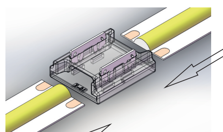
3.将灯带箭头示方向两边推入 Push the strip into the connector from both sides
