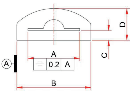
密封胶尺寸参考 Size reference after the strip light is glued
