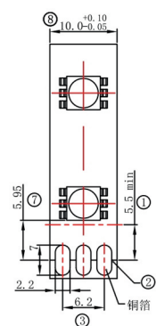
HR-S-SMD-3PIN-10MM
