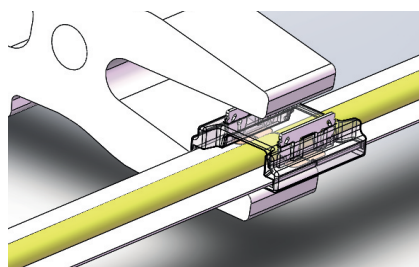
5.用钳子将端子夹入至塑胶面平齐(选用的工具夹口断应平整)，操作夹取为单边作业，夹入一边后再操作另一边 Use pliers to clamp the terminal to the level of the plastic surface, the operation is unilateral operation, clamp one side and then operate the other side.
